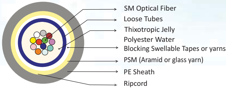
Cable cross-section
